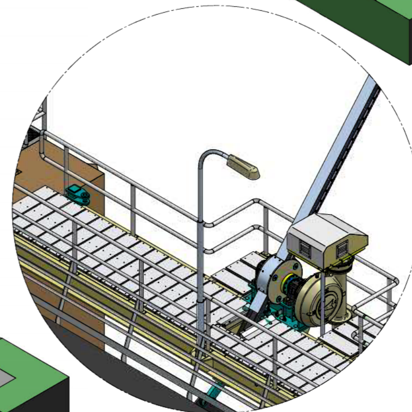
Detail PI 1201
